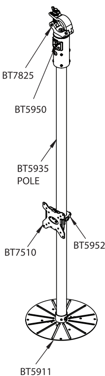
TRUSS MOUNT
