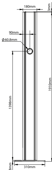
Front View
