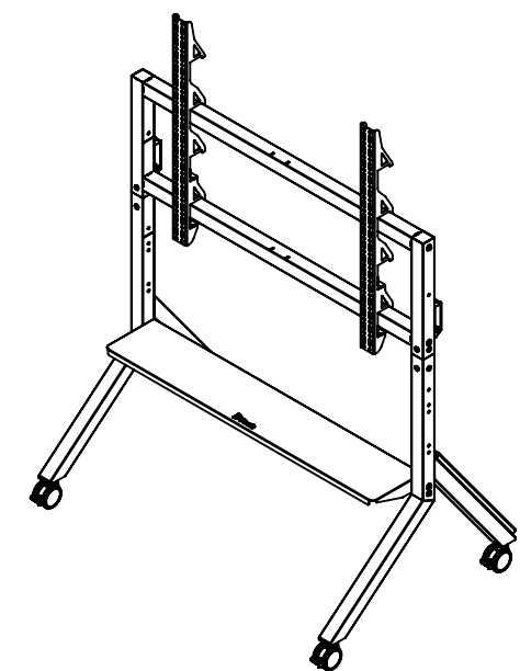
ISOMETRIC VIEW SCALE: 1 : 25
