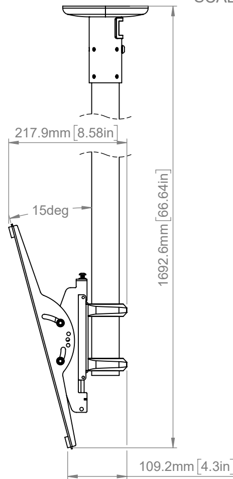
DETAIL A SCALE 1 : 3
