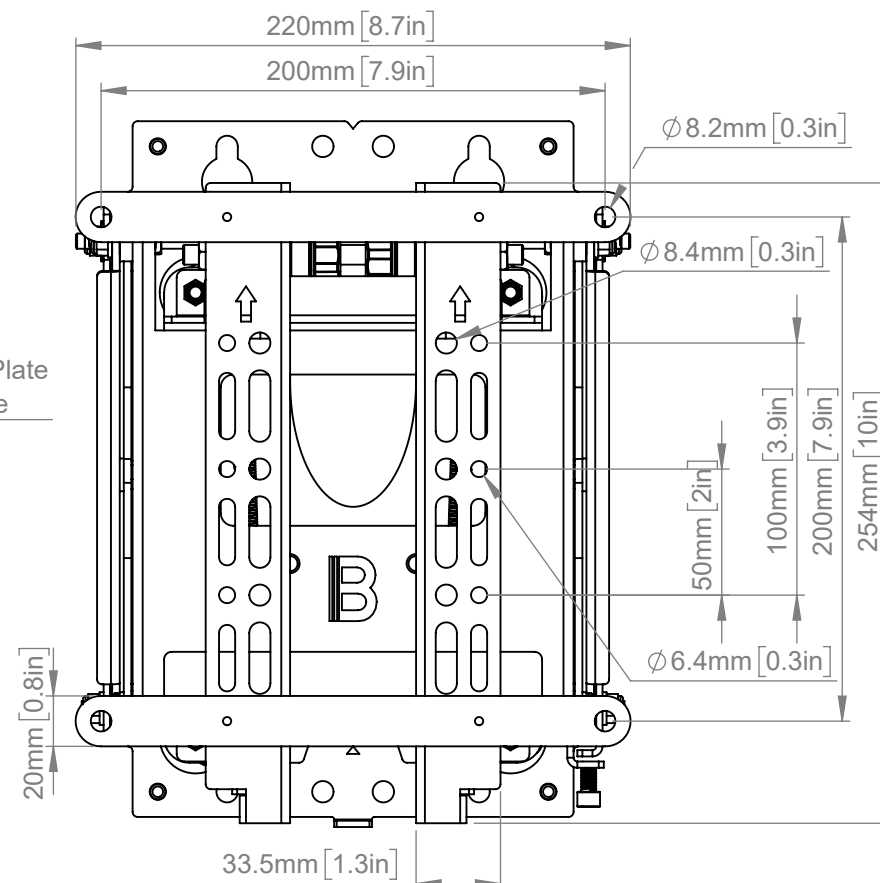
VESA 200 Adaptor Arms
