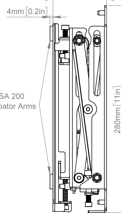
VESA 200 Adaptor Arms
