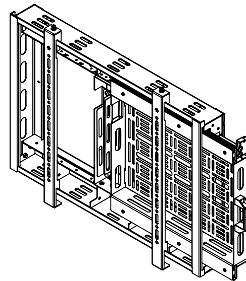
ISOMETRIC VIEW SLIDE OUT RIGHT CONFIGURATION SCALE: 1 : 10
