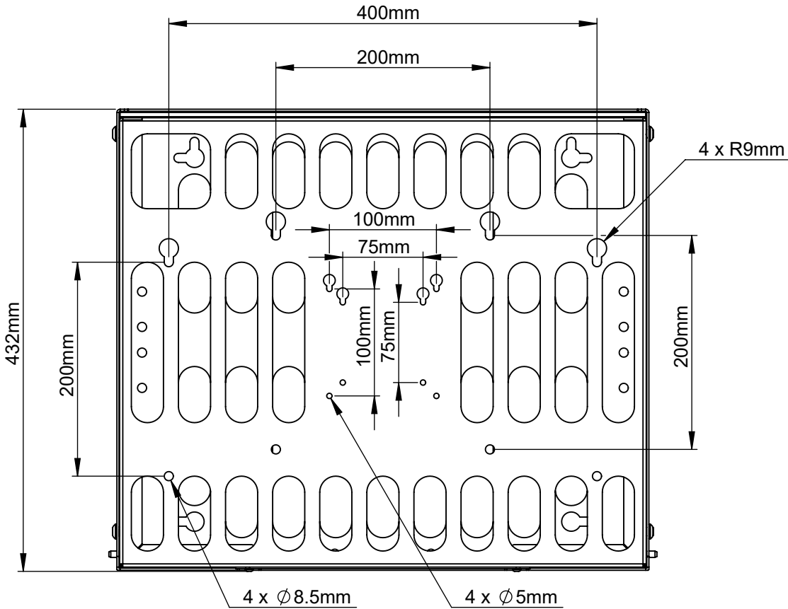
FRONT VIEW
