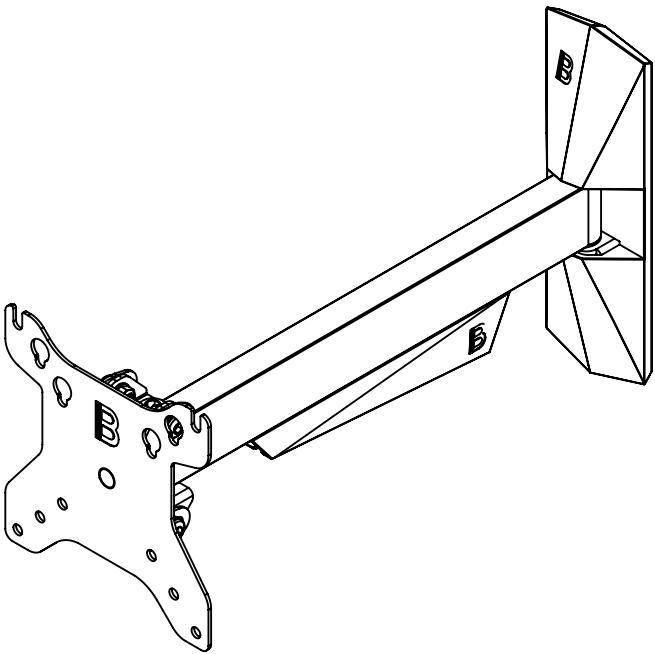
ISOMETRIC VIEW SCALE: 1 : 3
