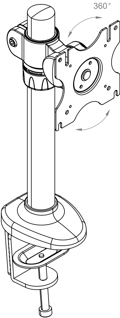
ISOMETRIC VIEW
