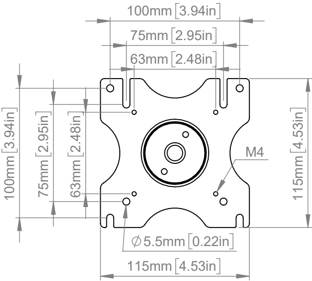
Interface Plate
