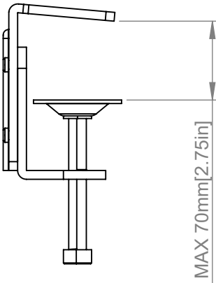
Desk Clamp
