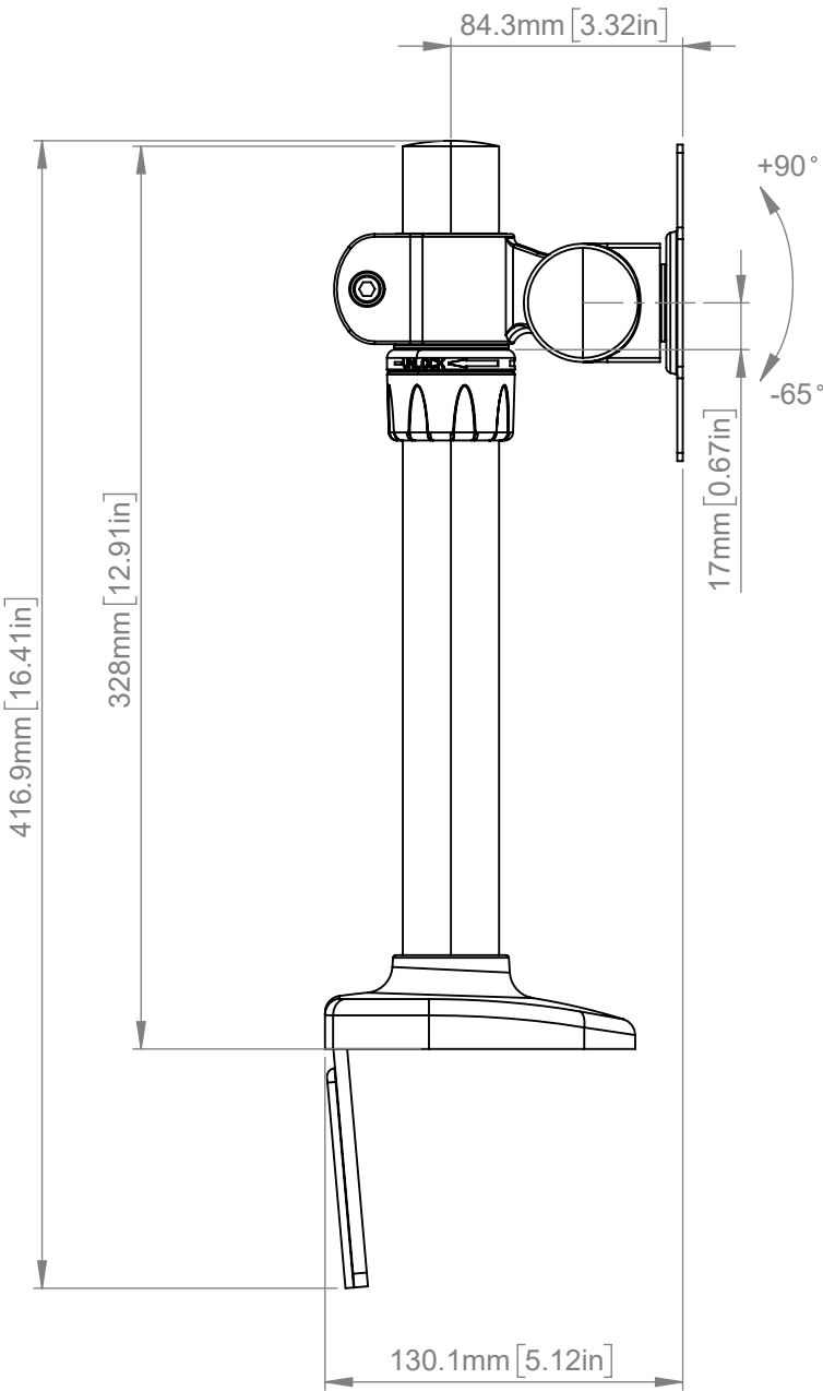
Side View
