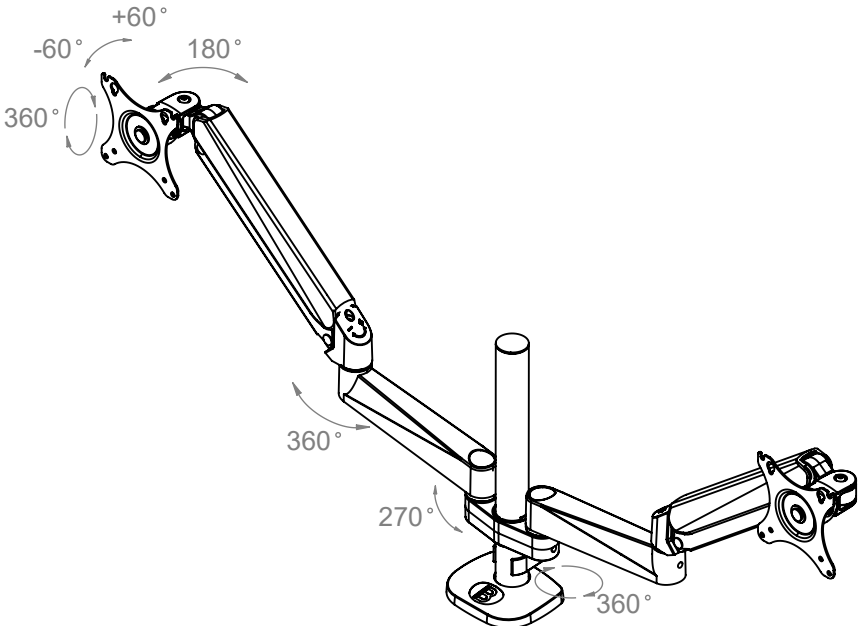
ISOMETRIC VIEW
