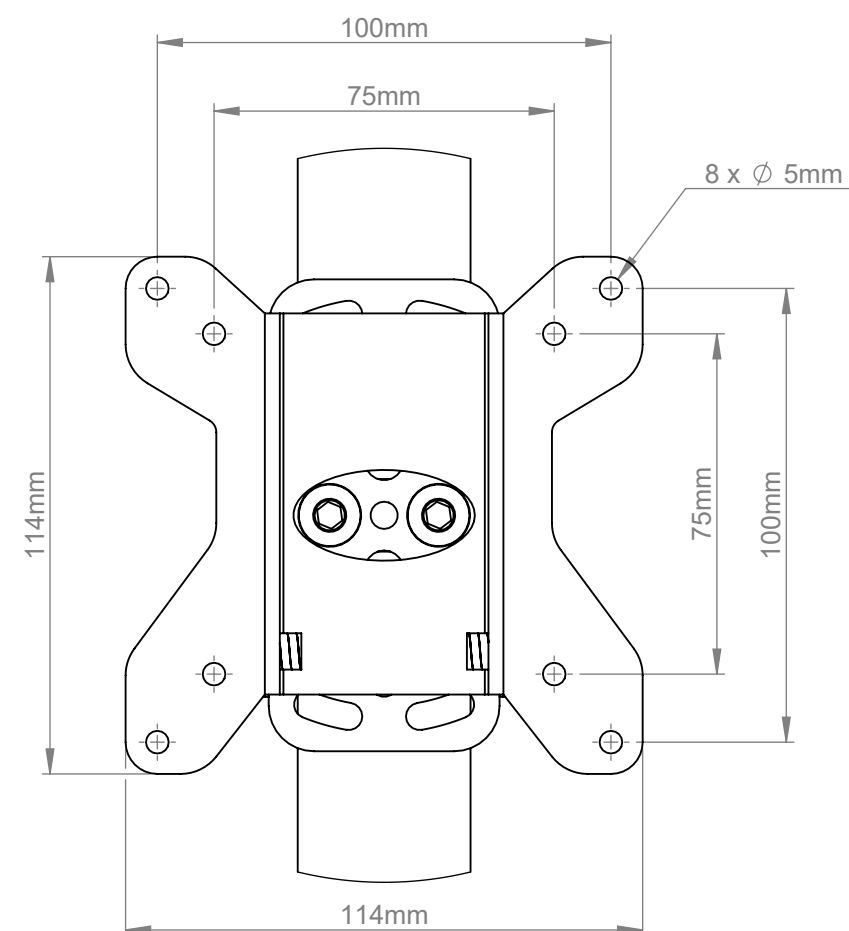
DETAIL C SCALE 3 : 5
