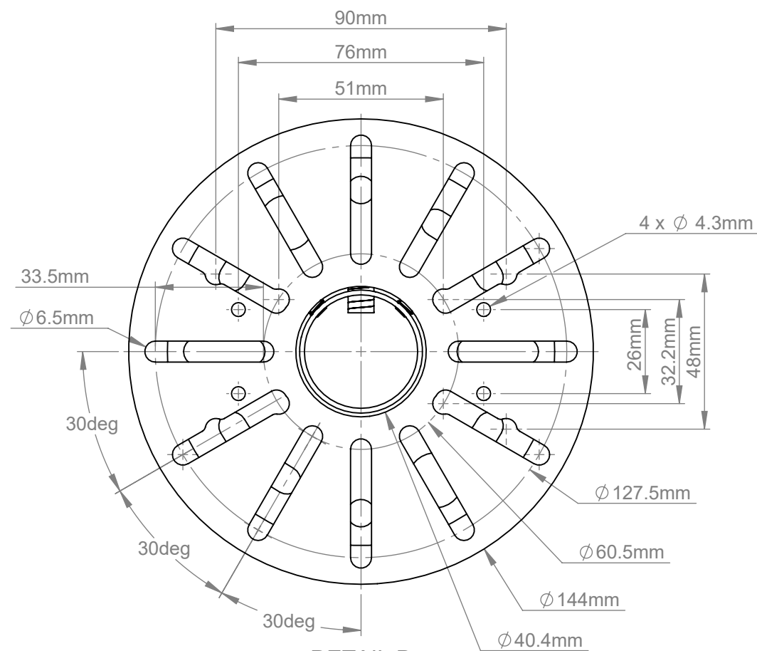
DETAIL B SCALE 3 : 5
