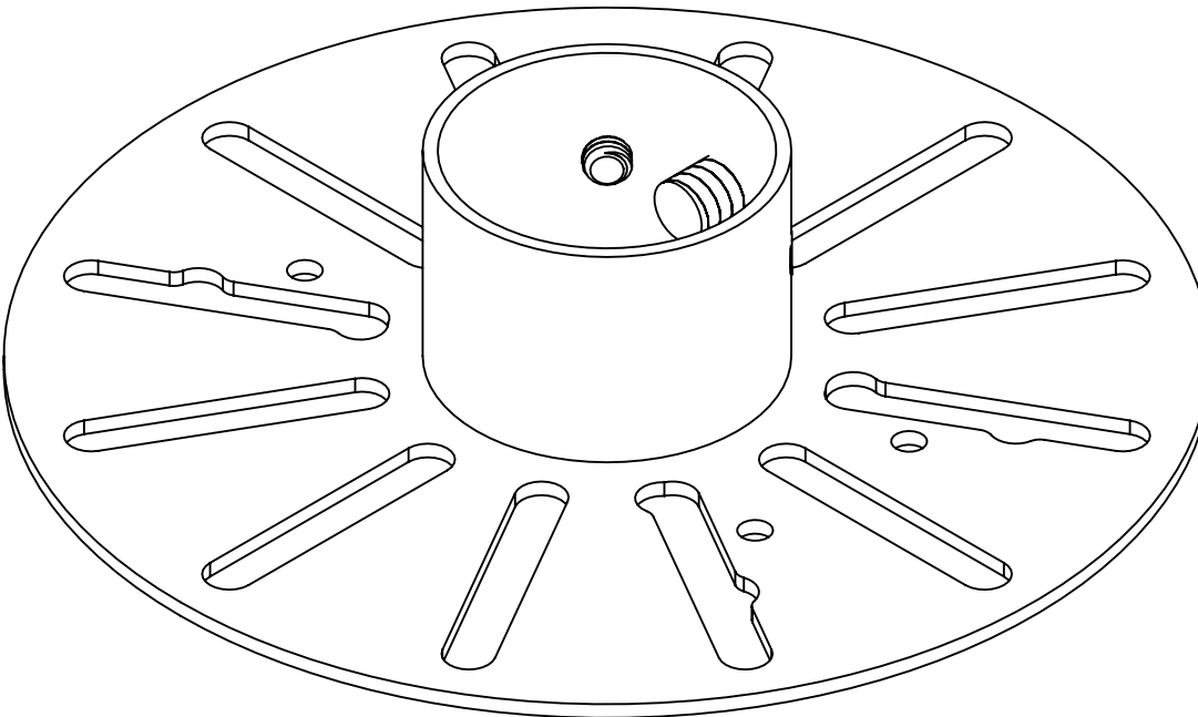
ISOMETRIC VIEW
