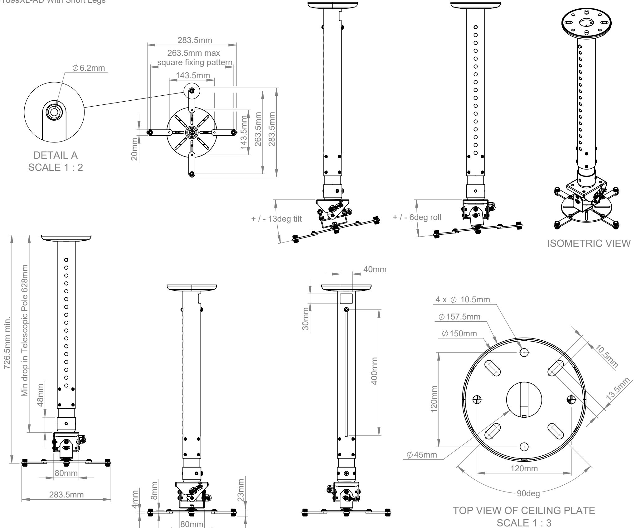
BT899XL-AD With Short Legs
