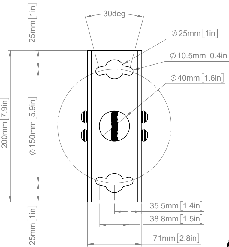
TOP VIEW OF CEILING PLATE SCALE 1 : 3
