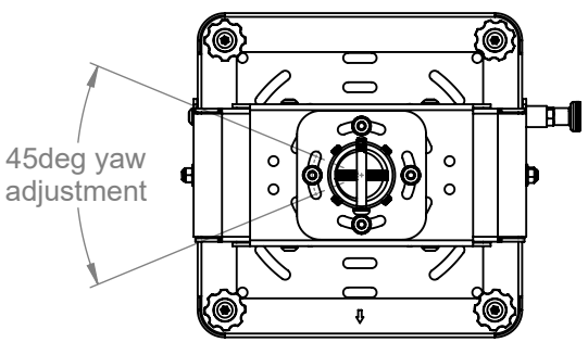
PROJECTOR MOUNT TOP VIEW
