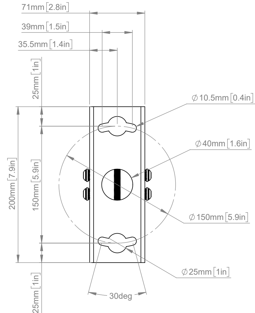
TOP VIEW OF CEILING PLATE SCALE 1:3
