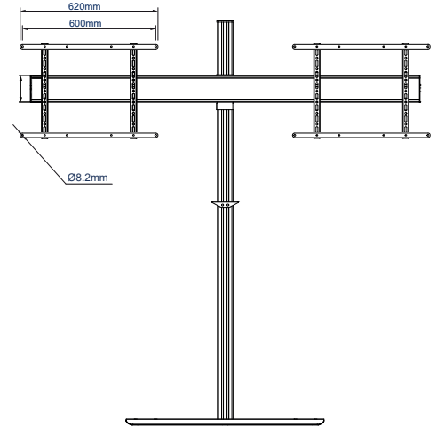
FRONT VIEW WITH ADAPTER ARMS
