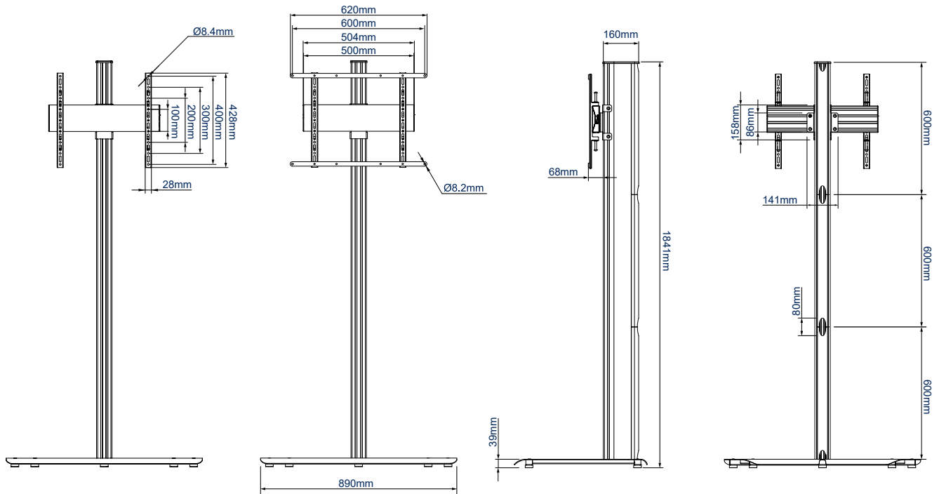
FRONT VIEW
