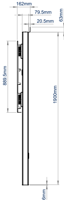
SIDE VIEW
