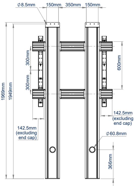
REAR VIEW
