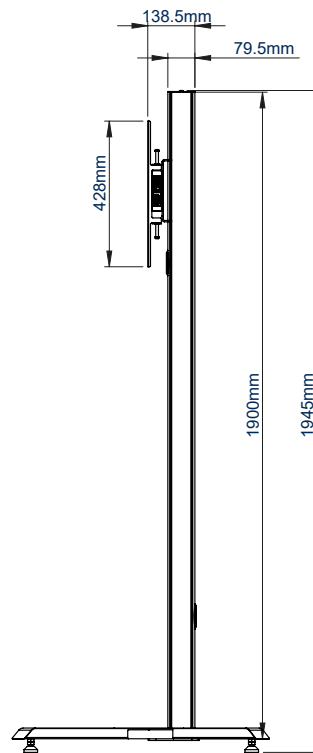
SIDE VIEW
