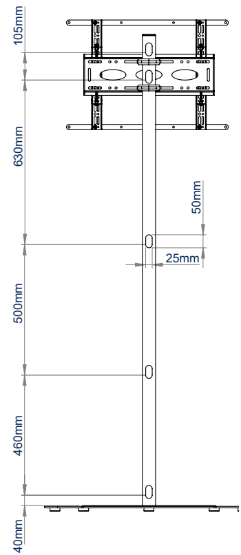
BACK VIEW
