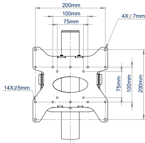
MOUNT
