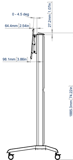
SIDE VIEW WITH MAX TILT
