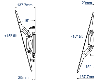
TILT RANGE
