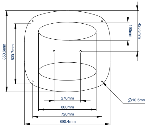
BASE VIEW
