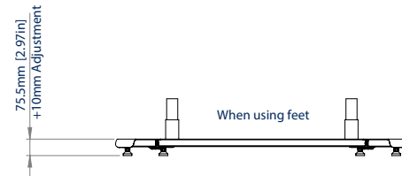
FRONT VIEW LEVELLING FEET
