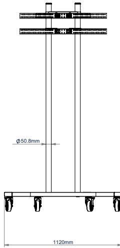
FRONT VIEW WITH CASTORS
