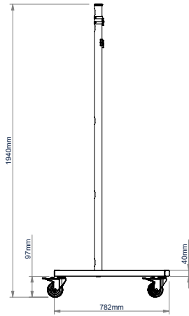
SIDE VIEW WITH CASTORS
