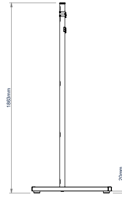
SIDE VIEW WITH ADJUSTABLE FEET
