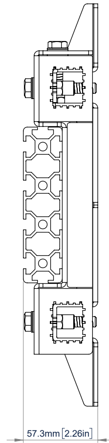
SIDE VIEW WITH BT8390 MOUNTING RAIL MINIMUM DEPTH
