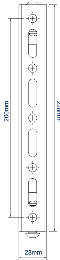
FRONT VIEW
