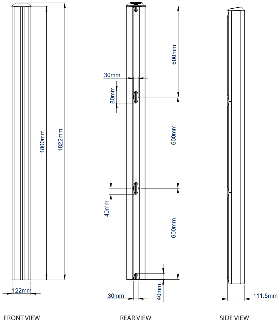
FRONT VIEW
