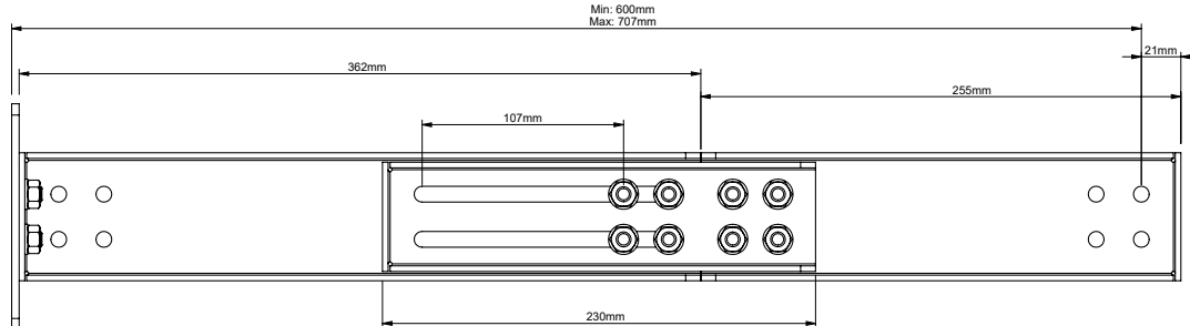
SIDE VIEW - CONNECTOR PLATE WITH LONG EXTENSION PLATE
