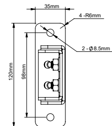
FRONT VIEW - WALL PLATE
