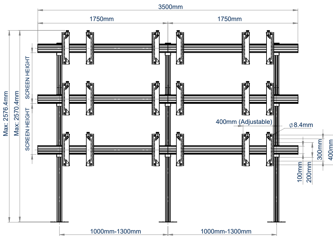
FRONT VIEW
