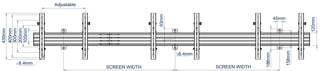
FRONT VIEW
