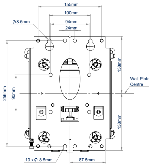
REAR VIEW WITH ADAPTOR ARMS
