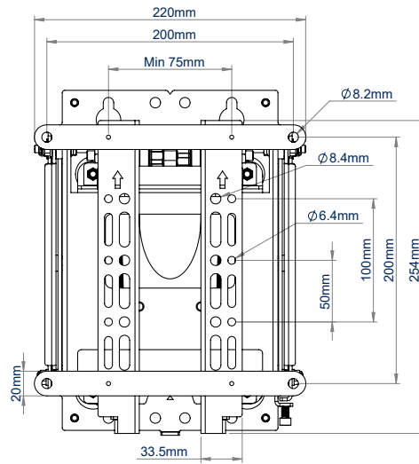
FRONT VIEW WITH ADAPTOR ARMS
