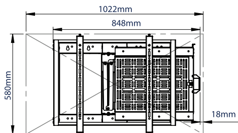
46" SCREEN CLOSED
