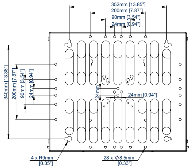
REAR VIEW
