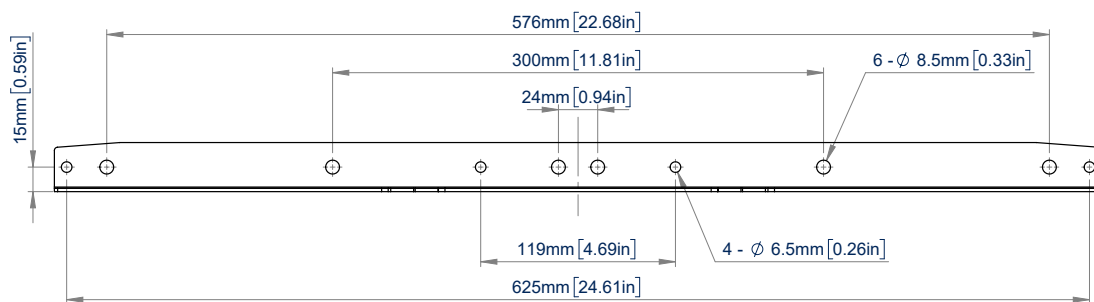
FRONT VIEW
