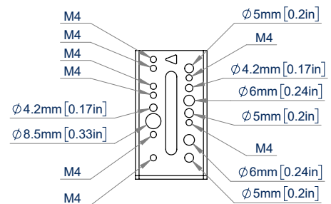
MOUNTING PLATE
