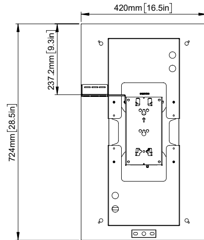
REAR VIEW PORTRAIT ORIENTATION WITH SAMSUNG 32" E-PAPER
