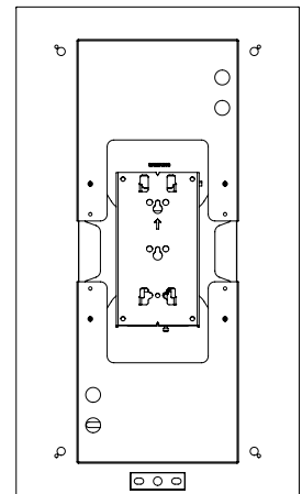
POSITION OPTION B FULL BUTTON ACCESS
