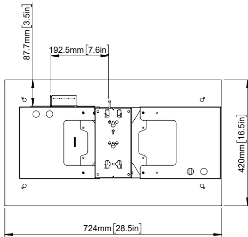
REAR VIEW LANDSCAPE ORIENTATION WITH SAMSUNG 32" E-PAPER
