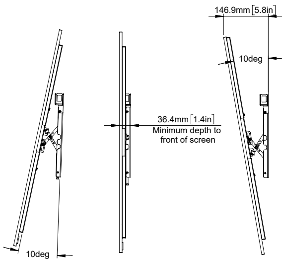
SIDE VIEW - TILT PORTRAIT ORIENTATION WITH SAMSUNG 32" E-PAPER
