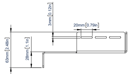
POWER BANK SIDE VIEW
