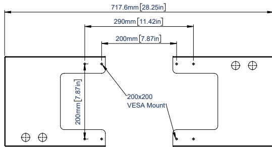
FRONT VIEW FOR COMPARTMENT PORTS
