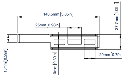
POWER BANK TOP VIEW
