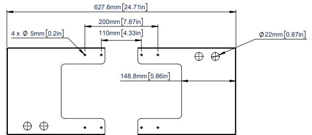
FRONT VIEW FOR DISPLAY BUTTONS
