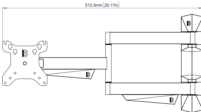
FRONT VIEW FLAT TO WALL
