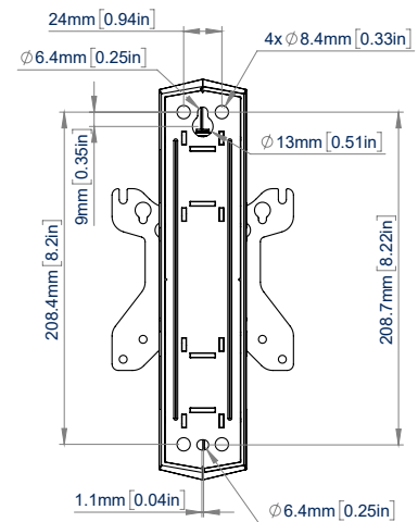
REAR VIEW WALL PLATE
