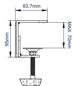
SIDE VIEW DESK CLAMP
