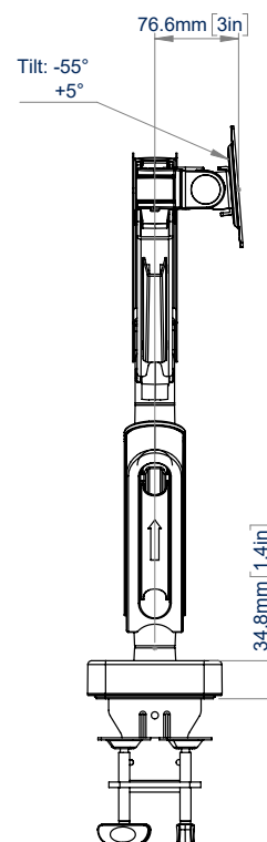
FRONT VIEW
