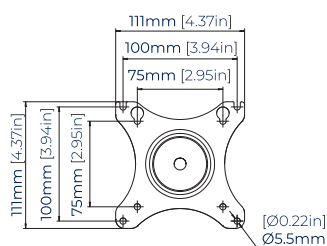
INTERFACE PLATE
