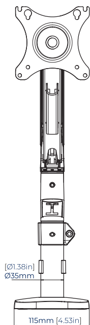
FRONT VIEW
