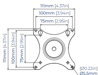
INTERFACE PLATE
