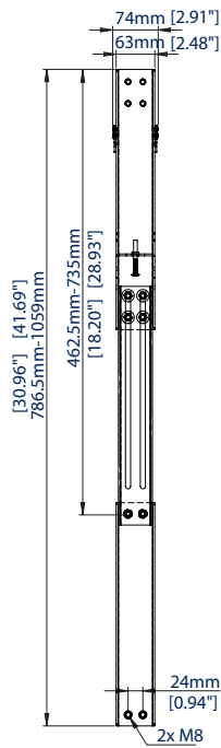
FRONT VIEW BELOW RAIL EXTENDED
