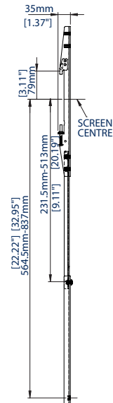
MOUNTING ON A BT9903
