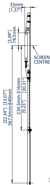
MOUNTING ON A BT8431 / BT8432 / BT8441 / BT8442
