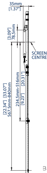
MOUNTING ON A BT8431 / BT8432 / BT8441 / BT8442
