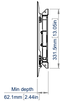
SIDE VIEW CLOSE-TO-WALL
