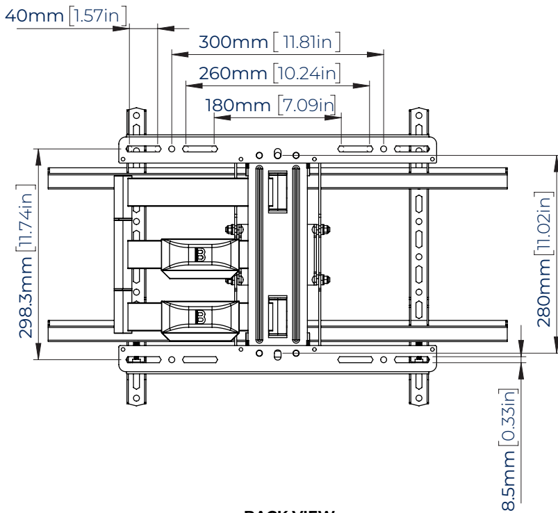
BACK VIEW
