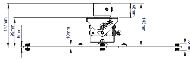
SIDE VIEW / FLAT WITH POLE ADAPTOR ATTACHED
