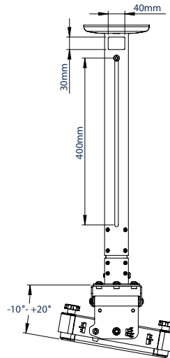
SIDE VIEW WITH INTERFACE TILT
