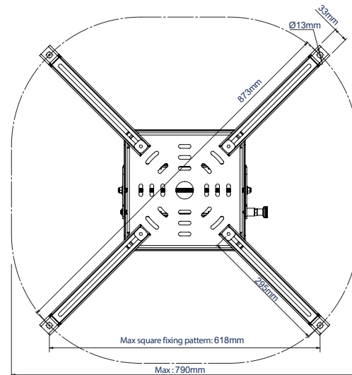
INTERFACE WITH LONG EXTENSION LEGS & SHORT EXTENSION LEGS
