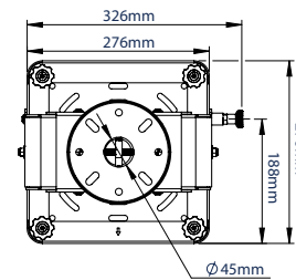
TOP VIEW WITH CEILING PLATE
