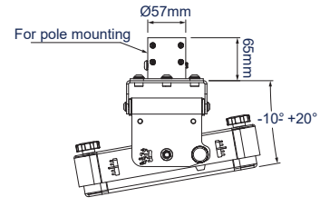
SIDE VIEW WITH INCLUDED POLE ADAPTOR
